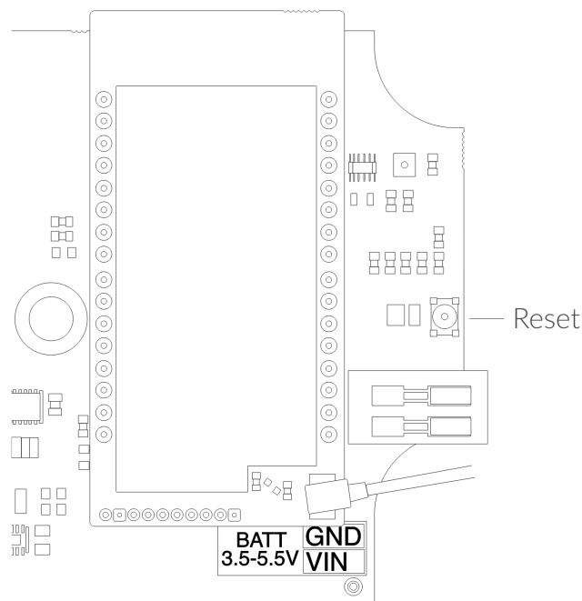
Figure 3 Reset button.
