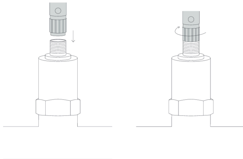
Figure 15 Connecting sensor instructions.
