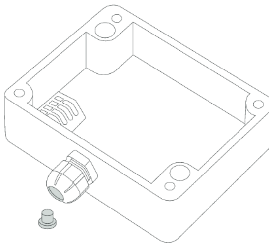
Figure 11 Device with removed top cover and PG7 cap marked.
