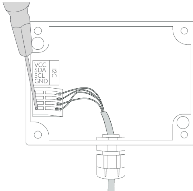
Figure 13 Connecting input cable instructions.
